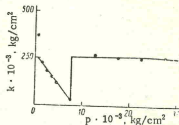
Fig. 2. Variation of the bulk compression modulus with pressure for \alpha - and \gamma -cerium.
